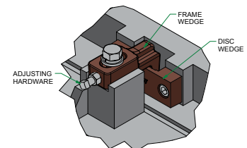
SIDE WEDGE SYSTEM
