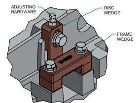
TOP AND BOTTOM WEDGE SYSTEM
