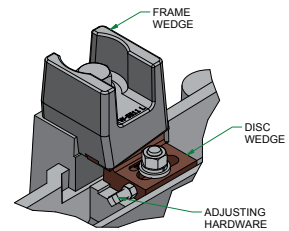
SIDE WEDGE SYSTEM
