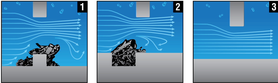
1. Raised seat wall traps debris 2. Recessed pocket seat traps debris 3. Q-Seal creates flow-through opening, no debris
