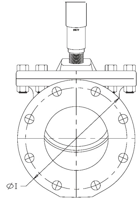
END VIEW
