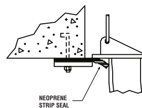
TOP SEAL DETAIL (BREASTWALL TYPE)
