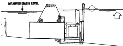
4. NORMAL HIGH TIDE GATE FULLY CLOSED
