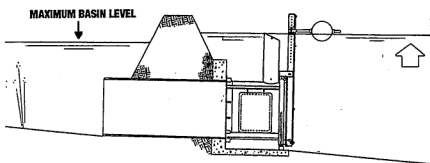
4. AT NORMAL TIDE LEVEL GATE IS CLOSED
